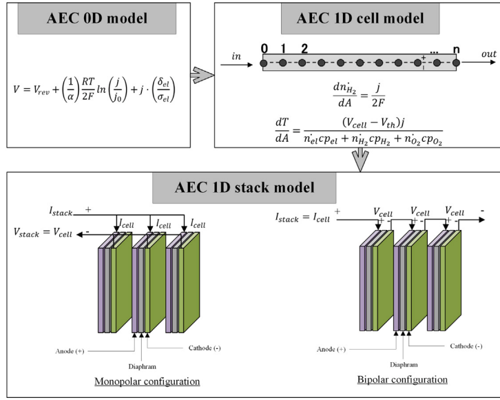
Fig. 3. Alkaline 1D stack model simulation flowchart. Starting with the single cell OD model, extended to the 1D cell model, solving mass and thermal balance, and finally 1D stack model, based on the electrical configuration among cells.
