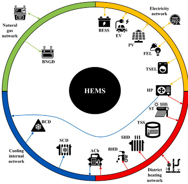
Fig. 6. Design architecture of proposed multi-carrier HEMS [28].
