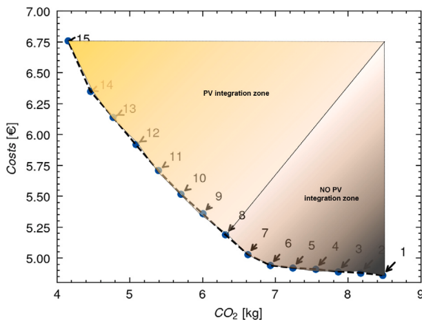
Fig. 11. The Pareto curve is derived from HEMS. In cases 1 to 8, there is no integration of PV systems, whereas in the remaining cases, PV systems are integrated, albeit at a higher economic cost.
