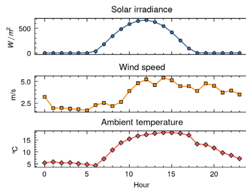
(c) Enviromental conditions variation during the operational day.
